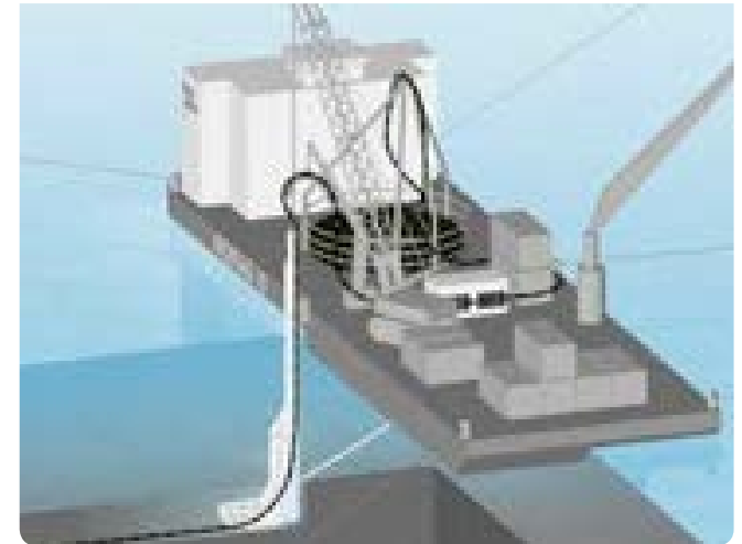
Figure 2-12 Schematic diagram showing the use of a jetting leg
