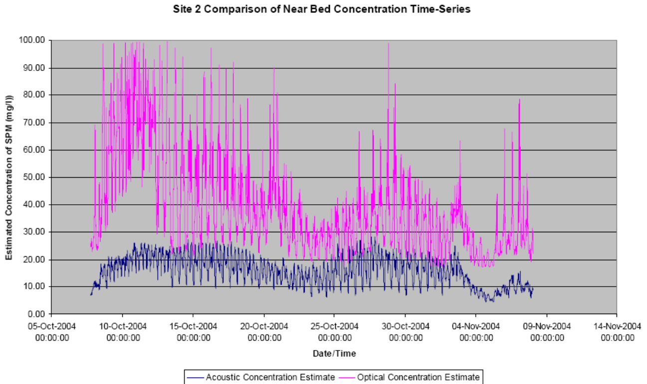
Figure 3-2 Time series of Near Bed SPM Concentration (SSC) determined by Optical Backscatter Sensor and Inversion of the Acoustic Backscatter Recorded by the Doppler Current Profiler at Site 2 (TES Ltd, 2004)
