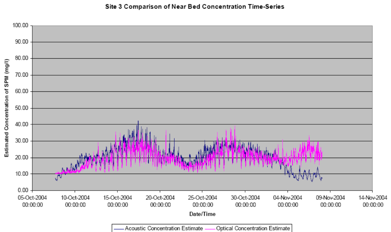
Figure 3-1 Time series of Near Bed SPM Concentration (SSC) determined by Optical Backscatter Sensor and Inversion of the Acoustic Backscatter Recorded by the Doppler Current Profiler at Sites 1 and 3 (TES Ltd, 2004)
