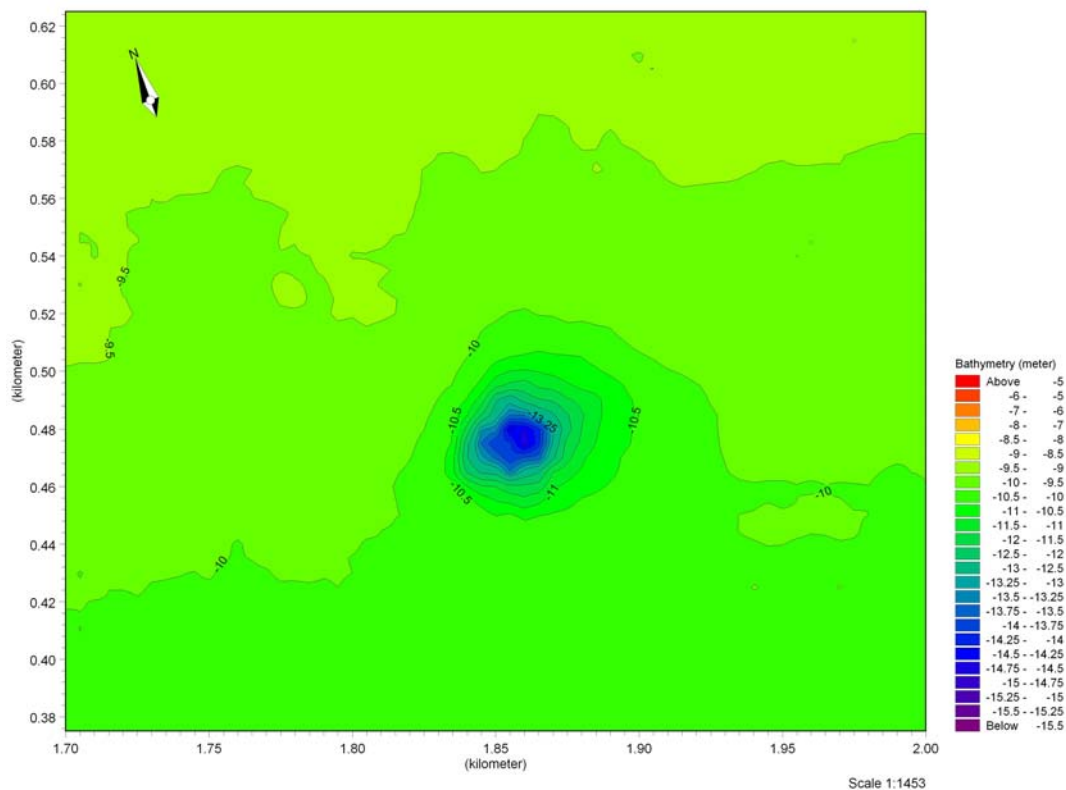
Figure 5-9 Scour hole formation around turbine foundation G5 (Robin Rigg), 2008 survey (26 March – 27 April 2008)
