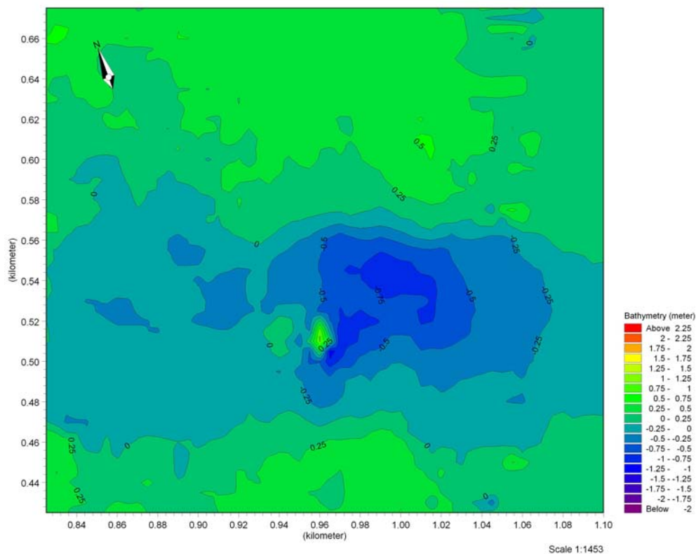
Figure 5-23 Difference in seabed levels at foundation position G3 (Robin Rigg) between December 2008 – January 2009 survey and March- April 2008 survey
