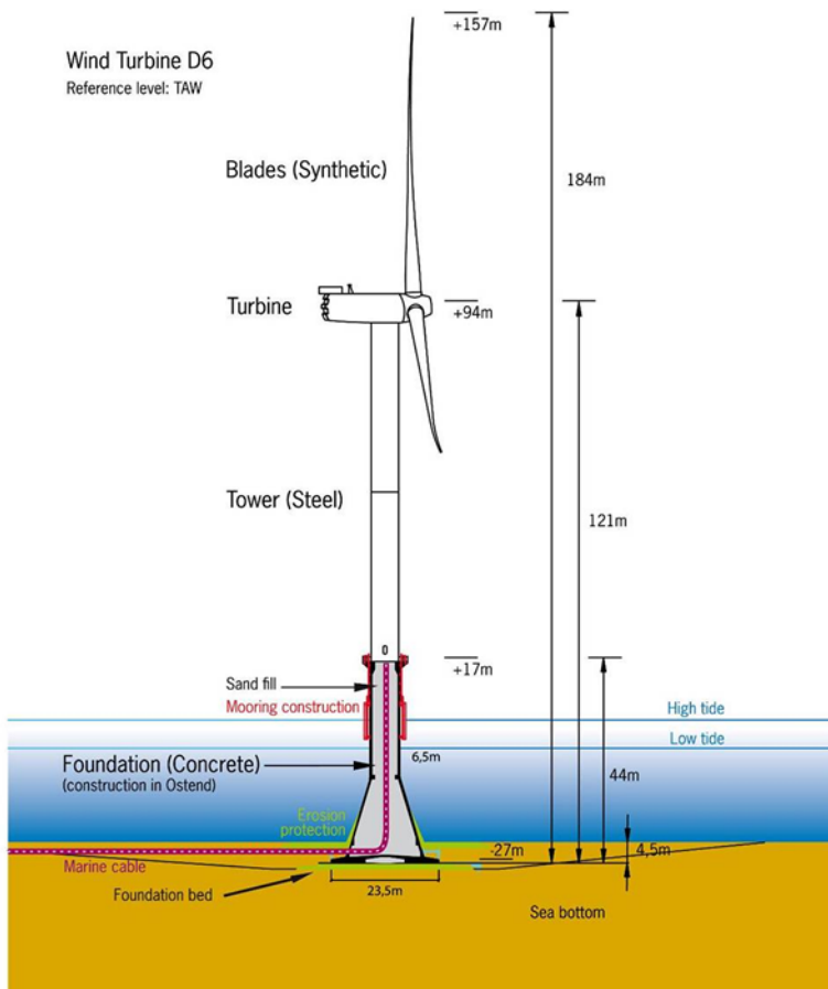
Figure 4-6 Schematic of the Thornton Bank GBF wind turbine design
