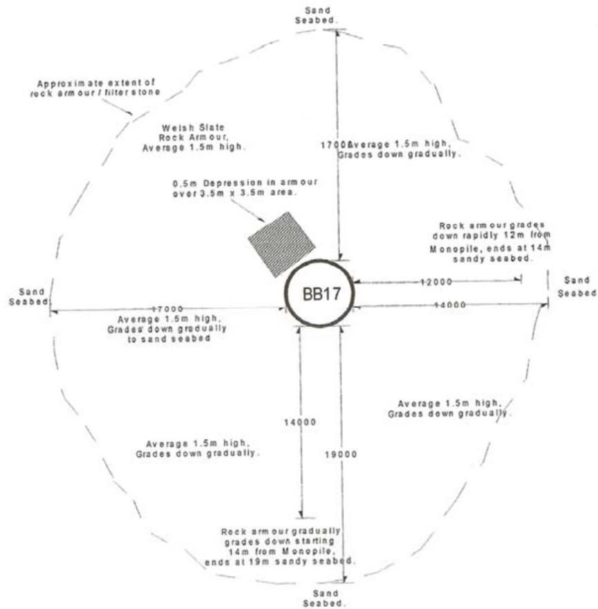
Figure 4-3 Scour protection extent at turbine BB17
