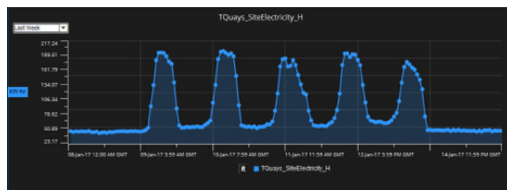
Fig.1 Typical well operated site weekly electrical demand profile
